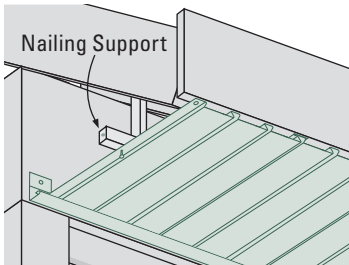
J-Channel
