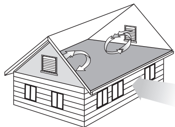
With wind blowing perpendicular to the ridge, the louvers act as both intake and exhaust vents.
